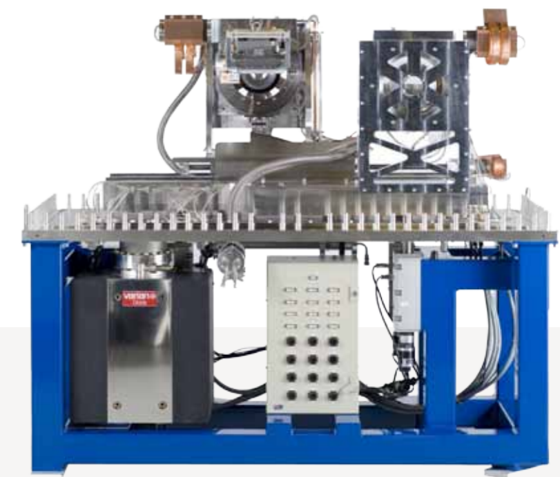
■ Double Crystal/Multilayer Monochromator (energy range ~ 8 ÷ 45 keV) for TOMCAT Beamline Swiss Light Source SLS Villigen (Switzerland)
